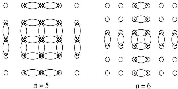
FIG. 2. Examples of saturated edges in array networks.
