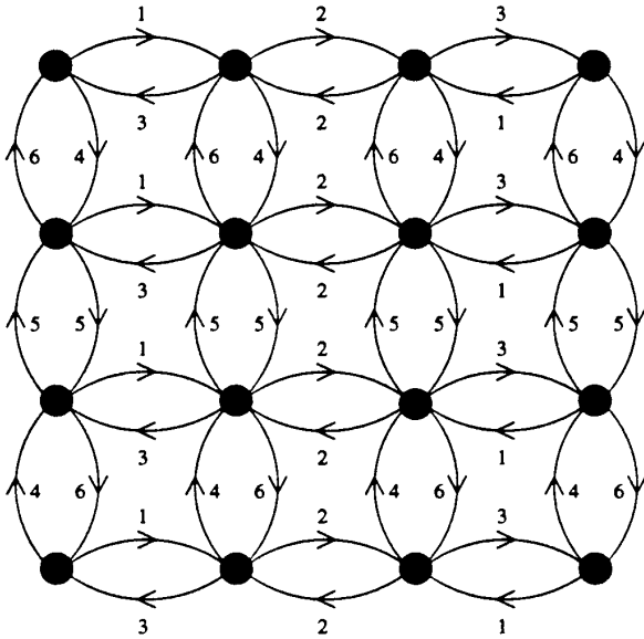
FIG. 1. Layering the array.
