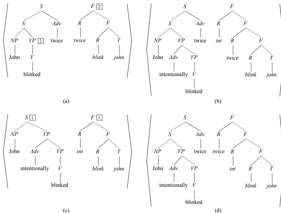
FIGURE 3. Derived tree pairs from the grammar of Figure 1. The derivation of the meaning int(twice(blink(j))) proceeds through the derived tree pairs in (a) and (b). The derivation of the meaning twice(int(blink(j))) proceeds through the derived tree pairs in (c) and (d).
