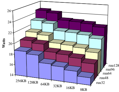
Figure 8: Power for gcc .
