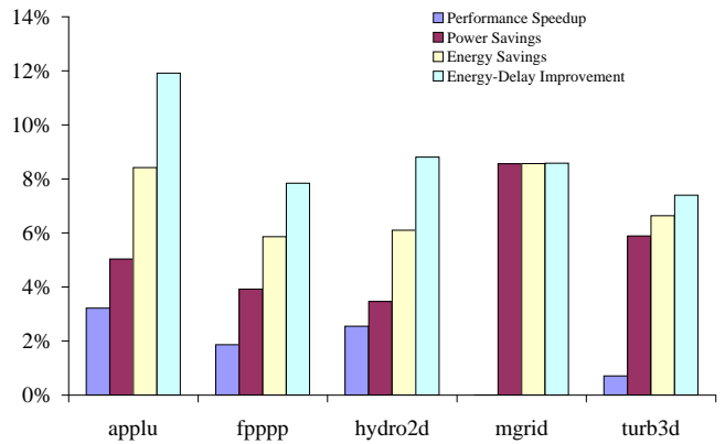
Figure 15: Performance and Power Effects of Memoing Technique.
