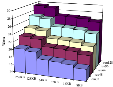
Figure 11: Power for turb3d .
