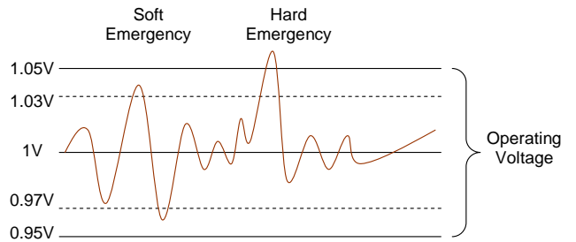
Figure 2: Soft and hard voltage emergencies.
