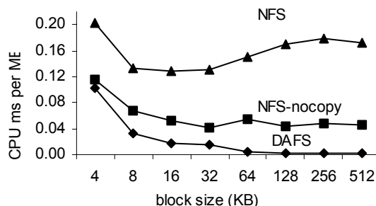
Figure 3. CPU ms per MB. No read-ahead.
