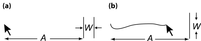
Figure 2. (a) In a classic Fitts’ law task, the constraint imposed by W is collinear to the movement axis. (b) In goal crossing, the constraint is orthogonal to the movement axis.
