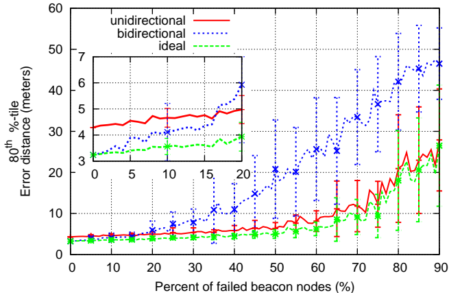
Robustness to Beacon Node Failure
