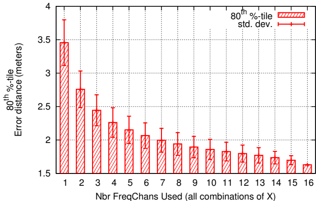
Error Distance vs. Nbr FreqChans Used txPowers= 0 dBm
