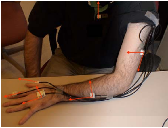
Figure 1 Sensor setup and orientation of the axes of the accelerometers.
