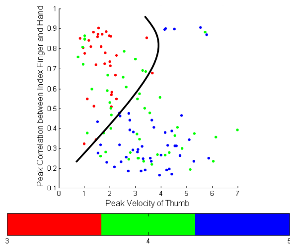
Figure 2 Scatterplot of peak correlation between accelerometer data from index finger and hand and peak velocity derived from thumb accelerometer data in comparison to Chedoke-McMaster Hand Stage scores. A line separates well samples associated with a score of 3 from samples associated with a score of 5. Samples for a score of 4 are in between and overlap with the rest of the data.
