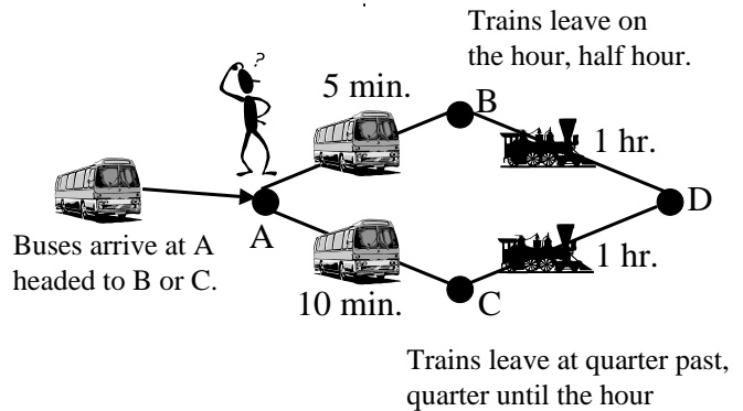
Figure 1: A basic bus and train network. Arrivals of buses from A to B and from A to C are each Poisson with an average wait of ten minutes. Travel times are constant. Trains from B leave on the hour and the half hour; trains from C leave fifteen and forty-five minutes into the hour.
