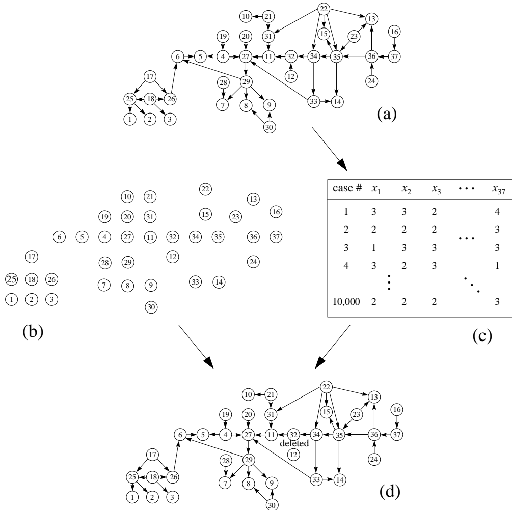
Figure 6: (a) The Alarm network structure. (b) A prior network encoding a user's beliefs about the Alarm domain. (c) A random sample of size 10,000 generated from the Alarm network. (d) The network learned from the prior network and the random sample. The only difference between the learned and true structure is an arc deletion as noted in (d). Network probabilities are not shown.
