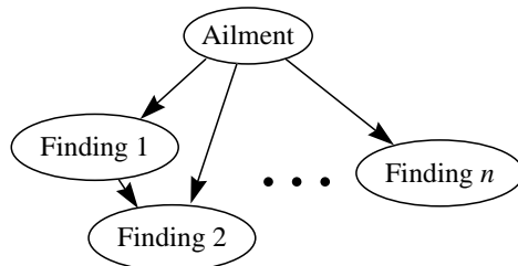
Figure 5: A Bayesian-network structure for medical diagnosis.
