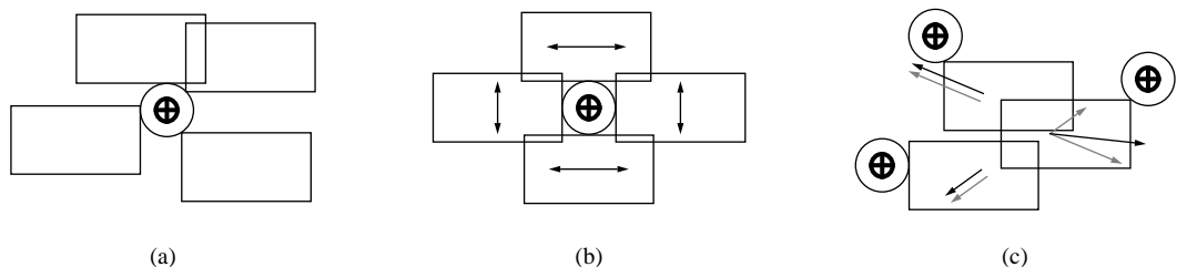
Figure 5: Some example potential label positions for Hirsch’s algorithm (a), along with the special zones (b), and an example of overlap vectors (c)
