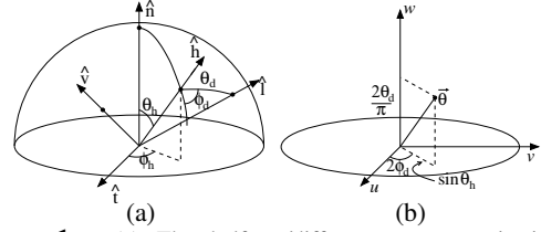
Figure 1: (a) The halfway/difference parameterization of Rusinkiewicz. In the isotropic case, the BRDF domain is parametrized by (\theta_h, \phi_d, \theta_d) [Rus98]. (b) The mapping defined by Eq. (1) that creates a parameterization suitable for interpolation.
