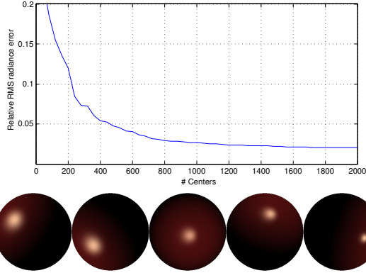
Figure 5: Top: Accuracy of the SBRDF recovered by reflectance sharing using the RBF representation in Eq. (6) as the number of centers is increased using a greedy algorithm. The input is 10 synthetic images of a hemisphere (five of which are shown) with linearly varying roughness.
