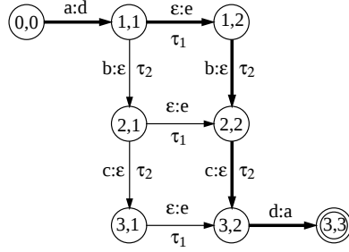
Figure 3: Composition with Marked \epsilon s
