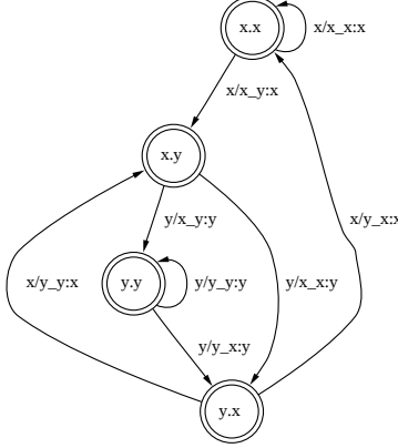
Figure 6: Context-Dependency Transducer
